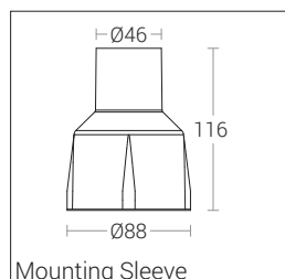
Mounting Sleeve
